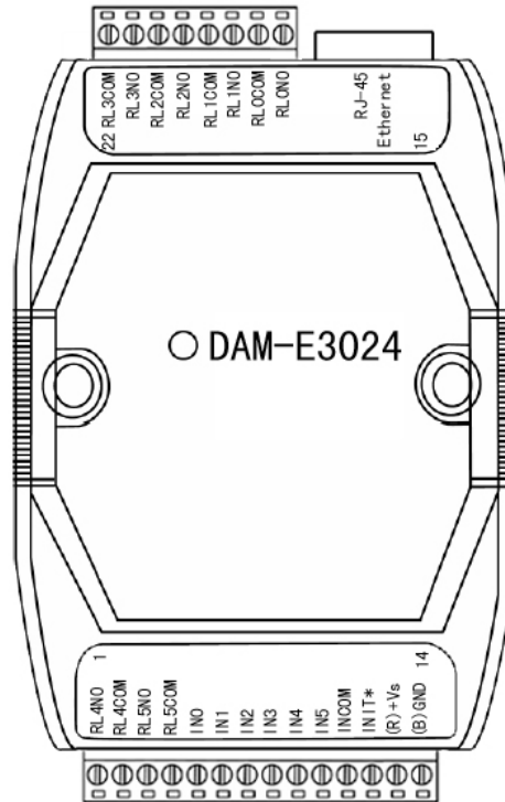
Fig.1 DAM-E3024 Drawing
